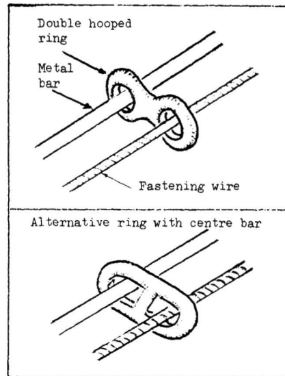
Sketch No. 2 SHEETED VEHICLES WITH SLIDING RINGS
