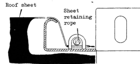
Sectional view
