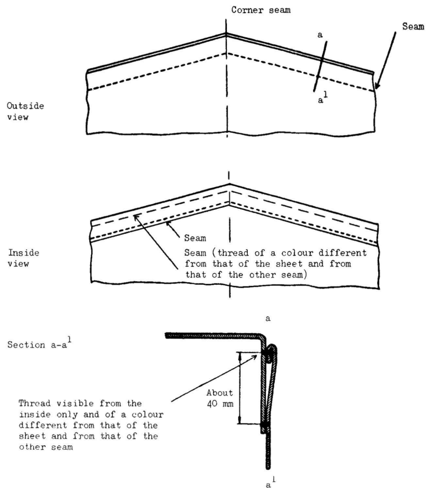
Sketch No. 2 SHEET MADE OF SEVERAL PIECES SEWN TOGETHER
