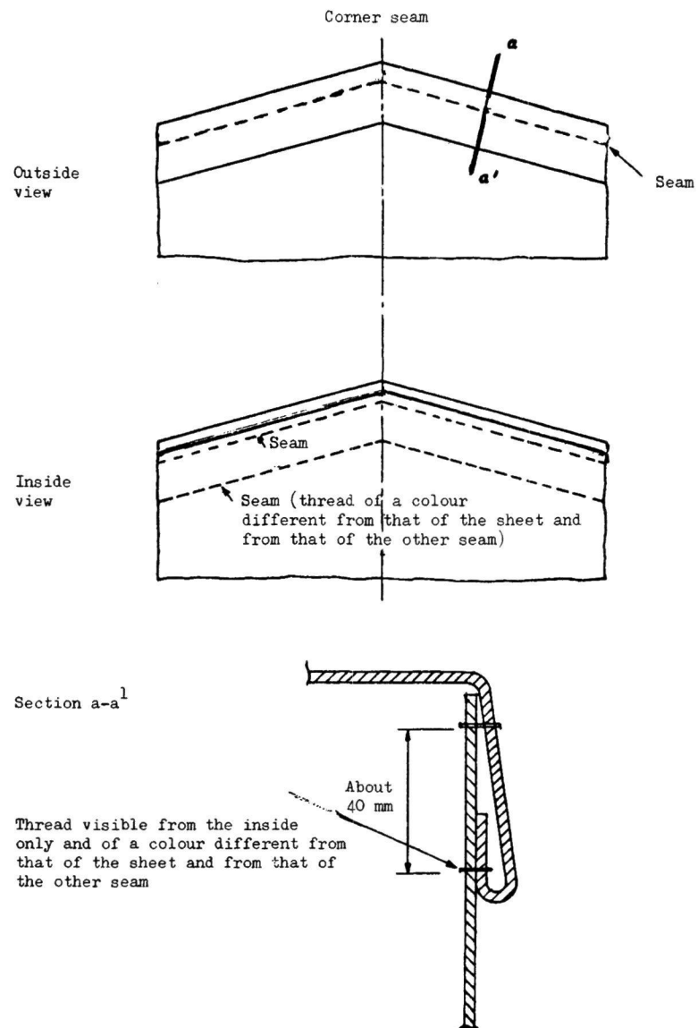
Sketch No. 2(a)
