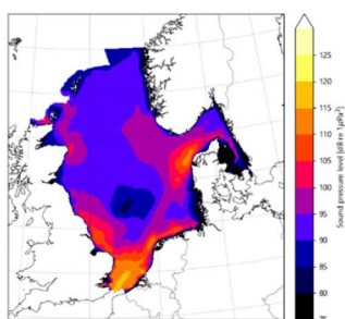
Figuur 11.4. Mediaan totale Sound Pressure Level, 125 Hz band.
