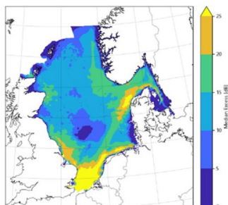
Figuur 11.5. Mediaan Excess Level, 125 Hz band.
