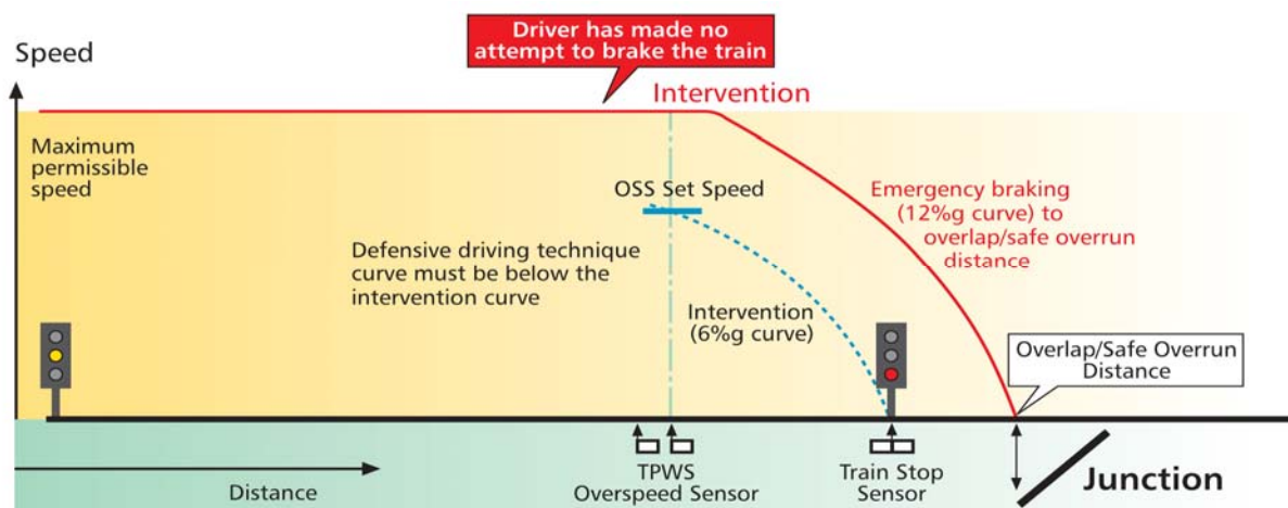
Figure 1 Basic arrangement of TPWS
