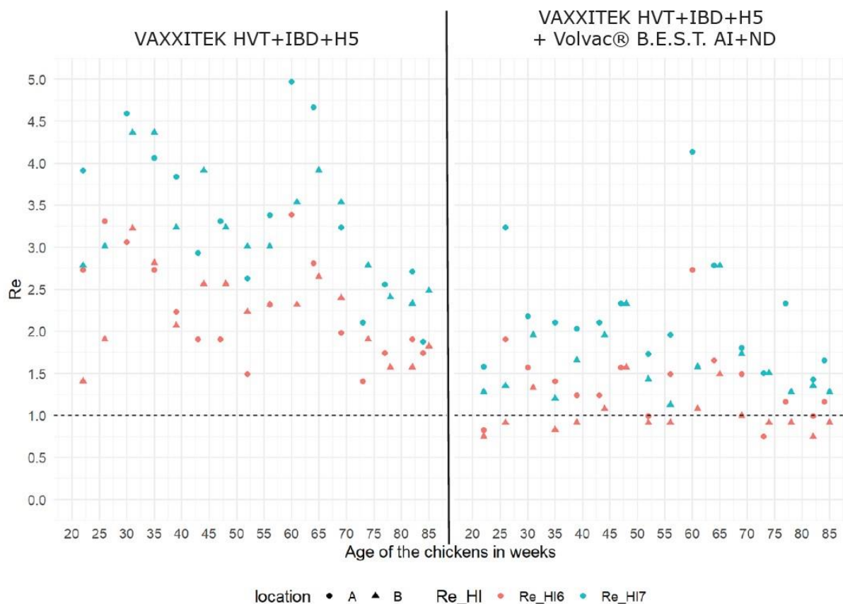
Figure 3.1 The effective reproduction number ( R_e ) estimated based on the fraction of chickens in the experimental groups (kept in the field) having high HI titers at each sampling time throughout the production cycle. These estimates were done for the models (with the lowest AICs) considering \log_2 HI titers: HI \geq 6 (red) or HI \geq 7 (blue) as cut-off values. The left panel shows the expected R_e for the experimental groups without booster vaccination whilst the right panel show these R_e values for the flocks receiving a heterologous to the prime booster vaccination. Dashed line indicates threshold value R_e = 1 .
