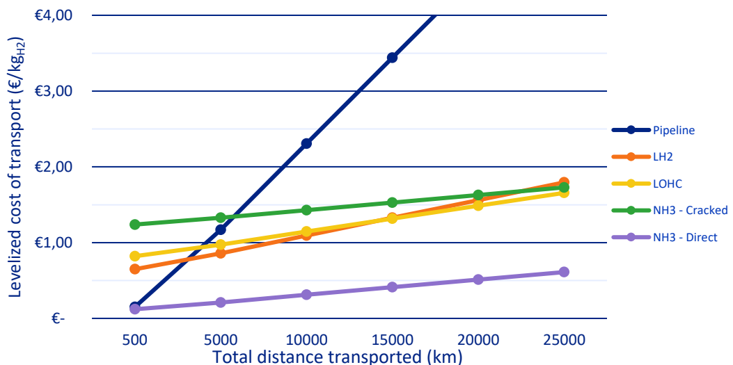
Figure 1.2: Cost comparison of hydrogen transport modes for different mediums 1 , adapted from (Ortiz Cebolla, Dolci, & Weidner, 2022). The pipeline transports compressed H 2 , the remaining carriers are all transported by maritime shipping. The hydrogen transport costs are levelized based on the hydrogen content for each carrier. For direct ammonia, this means the levelized cost are calculated using the hydrogen content of ammonia.
