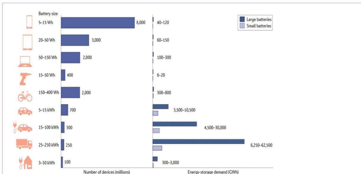
Estimates of the number of battery packs (large and small) produced from 2016 to 2050, in the researchers' scenario. Source: Vaalma et al., Nature Reviews Materials, 2018.
