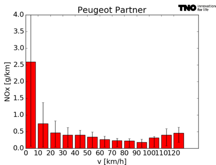
Figure 3-1: Average NO x emissions of a Peugeot Partner Euro 6 diesel per velocity bin for all trips. The error bars represent +/- one standard deviation from the median. Idling is excluded.
