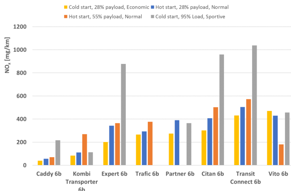
Figure 3-62: NO x emissions of RDE trips with different payloads and driving styles of 8 vehicles
