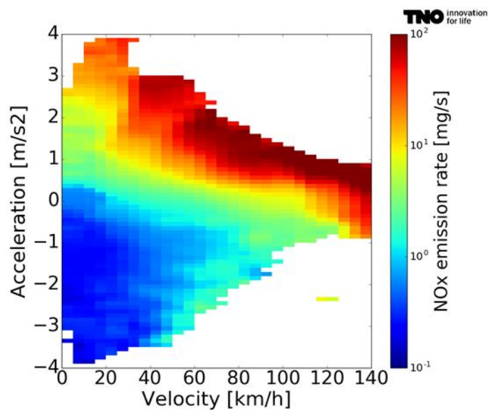
Figure 3-9: NO x emission rate [mg/s] of a Ford Transit Connect Euro 6 diesel in bins of velocity and acceleration.
