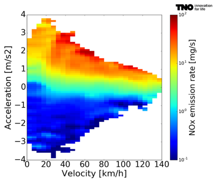
Figure 3-6: NO x emission rate [mg/s] of a Renault Trafic Euro 6 diesel in bins of velocity and acceleration.
