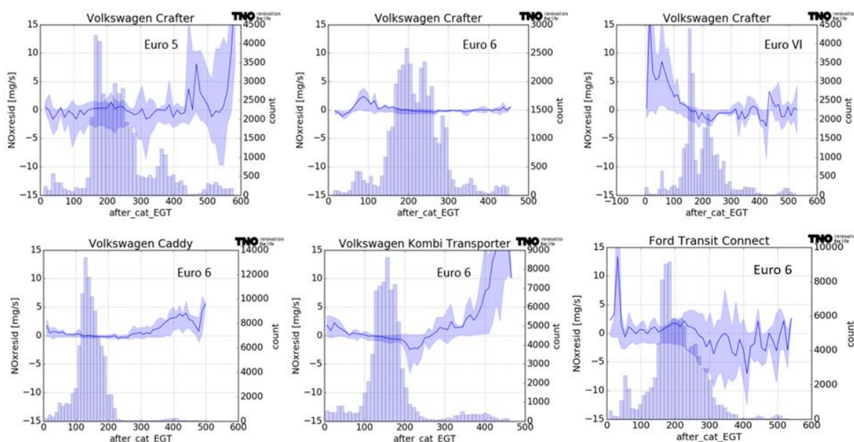
Figure 4-2 Residual \text{NO}_x emission per vehicle (in mg/s, left axis) with respect to the prediction from a parameterization using velocity and \text{CO}_2 , plotted against the exhaust gas temperature. The shaded band reflects the standard deviation. The histogram displays the number of seconds of data available in each temperature bin (right axis).
