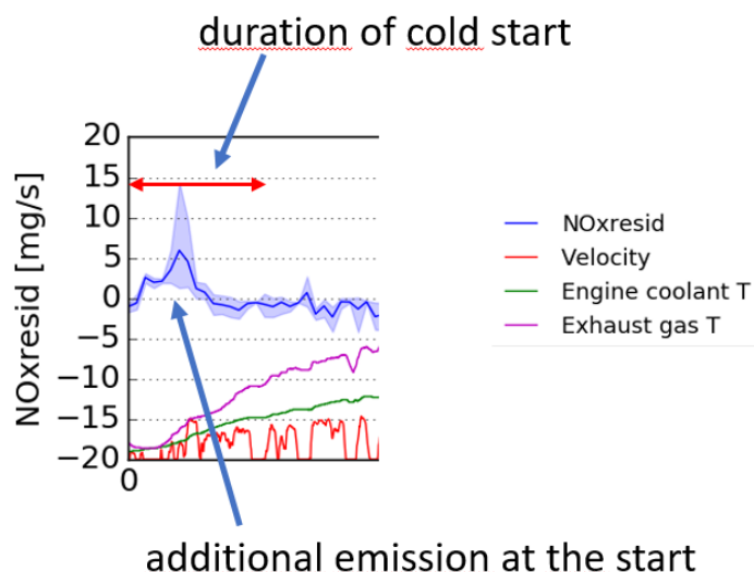
Figure 4-3: A detail plot of the time-dependent residual analysis: A clear initial peak of additional emissions is seen which decreases while the temperatures ECT and EGT increase. The area under the blue line yields the total estimated cold start contribution.
