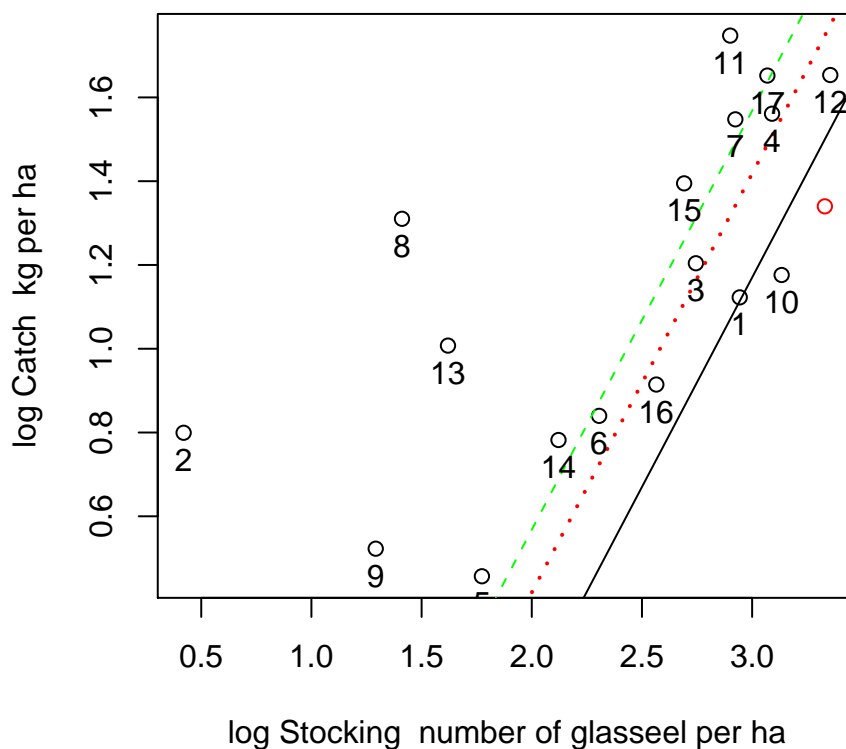
Figure 5: Yield per ha plotted against number of glasseels stocked per ha for the different areas, each indicated by a randomly generated number. Lines show model predictions. The green dashed line shows the maximum yield of silver eel per glasseel, if silver eel fisheries is 100 % efficient, that is if f = 1 . The red dotted line gives the maximal yield of yellow eel of 26 g per glasseel if the minimum size is 38 cm. The black solid line gives a yield of 14.8 g per glasseel which is equal to 40% of the maximal silver eel catch.
