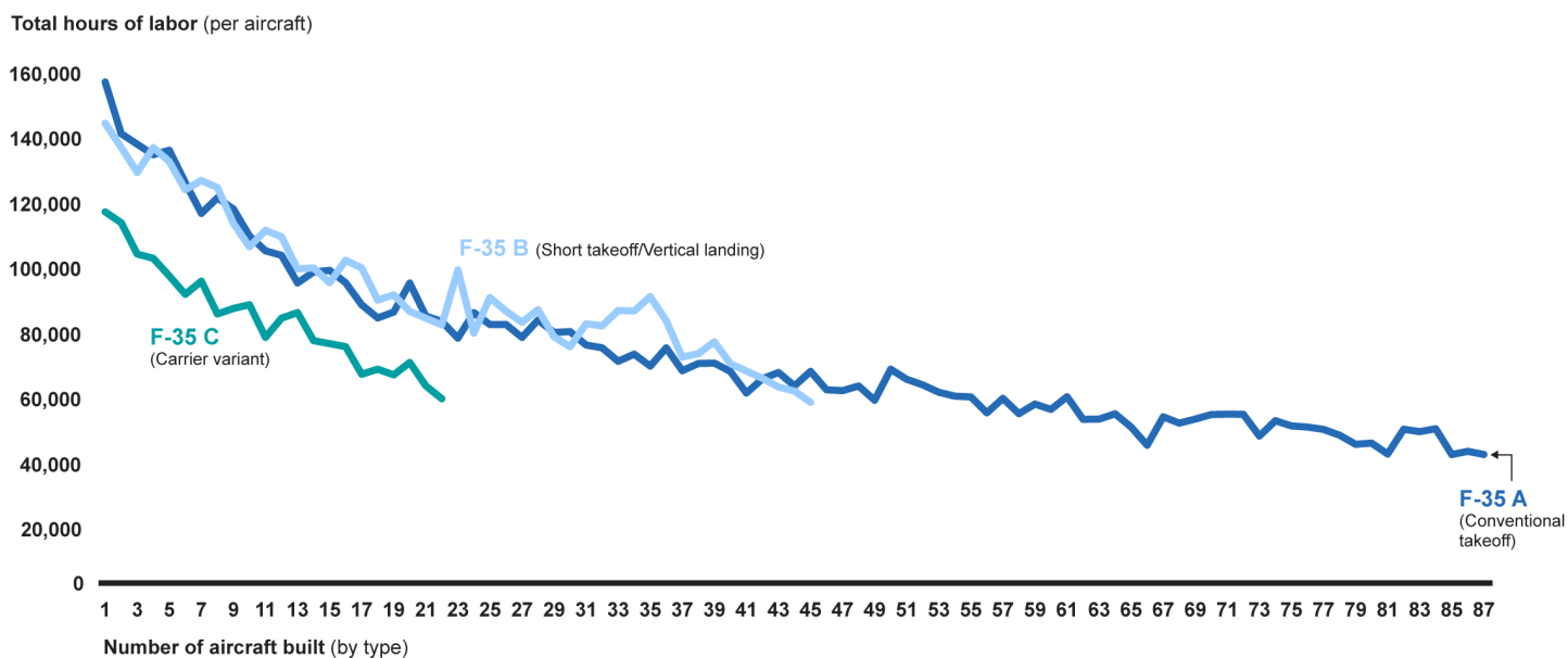
Figure 6: Trend in Labor Hours to Build F-35 Joint Strike Fighter Aircraft by Variant
