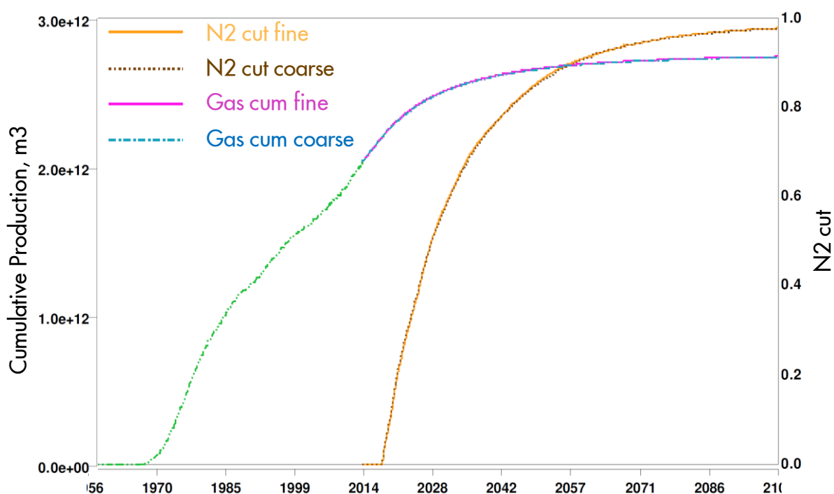
Figure 12.13 Sensitivity of nitrogen injection for the grid size used in the reservoir simulation. Both the gas production and the nitrogen cut at the producer wells are not significantly affected by the cell dimensions.
