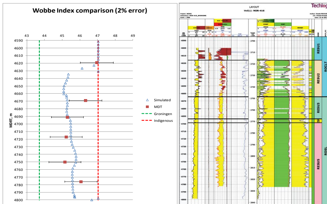
Figure 12.4 The experience with these models gives additional confidence in the modelling of the nitrogen displacement process in the Groningen field.
