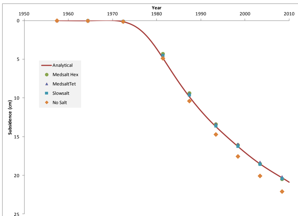
Figure 4.15 Subsidence versus time in the NW aquifer ( x=237000 y=603000 ) for Geomec models and analytical model (Geertsma and van Opstal)
