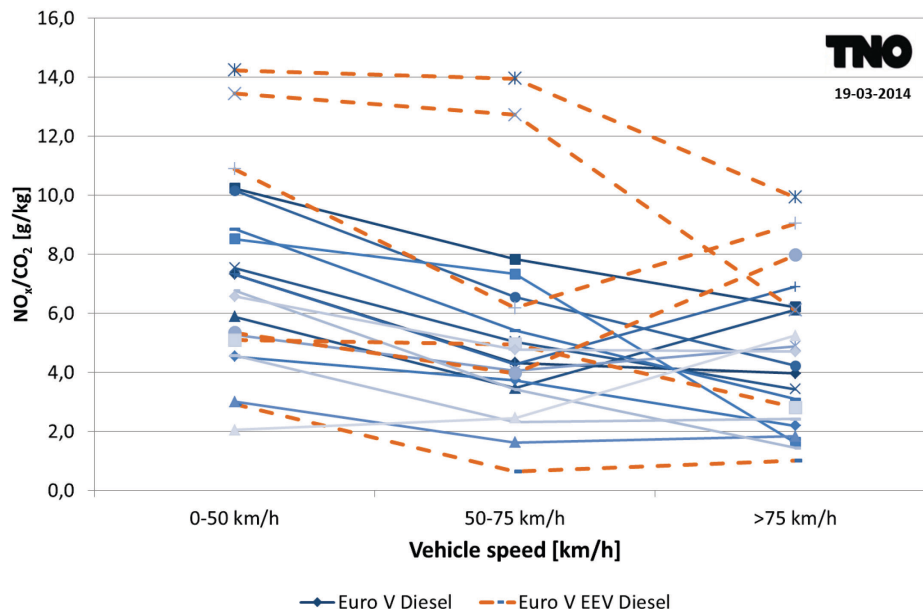
Figure 12: CO 2 specific \text{NO}_x emissions of the tested vehicles with Euro V and Euro V EEV diesel engines, over three different speed ranges. The lines between the speed intervals are to distinguish individual vehicles and their trends of \text{NO}_x emission over three speed ranges.
