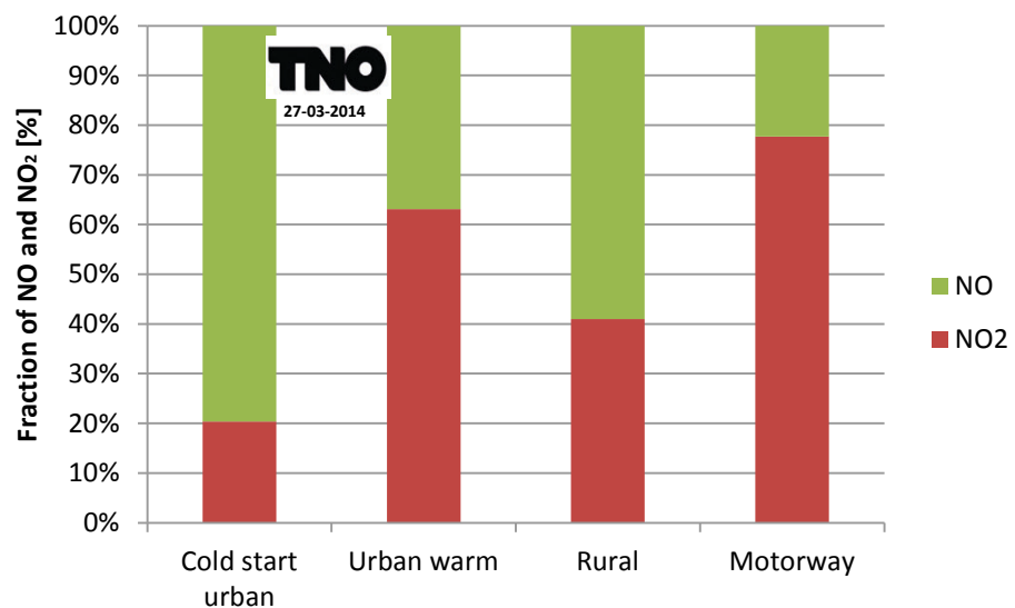
Figure 19: \text{NO} and \text{NO}_2 fractions in the \text{NO}_x emission of the Euro VI heavy-duty diesel vehicles, averaged for all vehicles and per type of operation.
