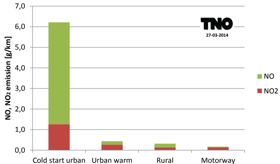
Figure 18: \text{NO} and \text{NO}_2 emissions of the Euro VI heavy-duty diesel vehicles, averaged for all vehicles and per type of operation. \text{NO} and \text{NO}_2 are calculated as \text{NO}_2 equivalent.
