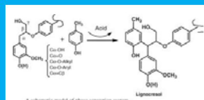
Fig. 1 Lignocresol (Bron: Funaoka)
