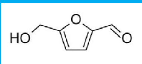
Fig. 1 Hydroxymethylfurfural (Bron: zie ref. 1)
