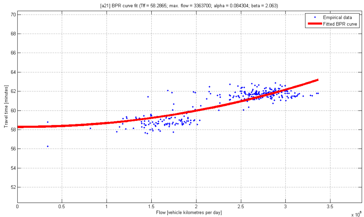
Figure 33: E34 between interchange Ranst and Dutch border
