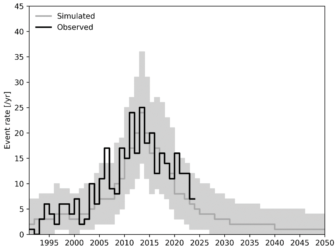
Figure 1 Calibration of the seismological model based on the earthquakes with a magnitude M_L \geq 1.5 until 1 January 2024.
