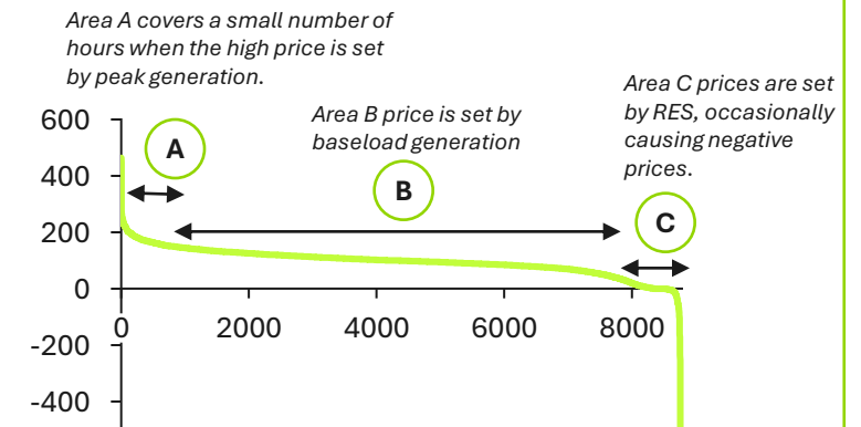
Figure 17: Illustrative price duration curve [EUR/MWh] for NL¹.
