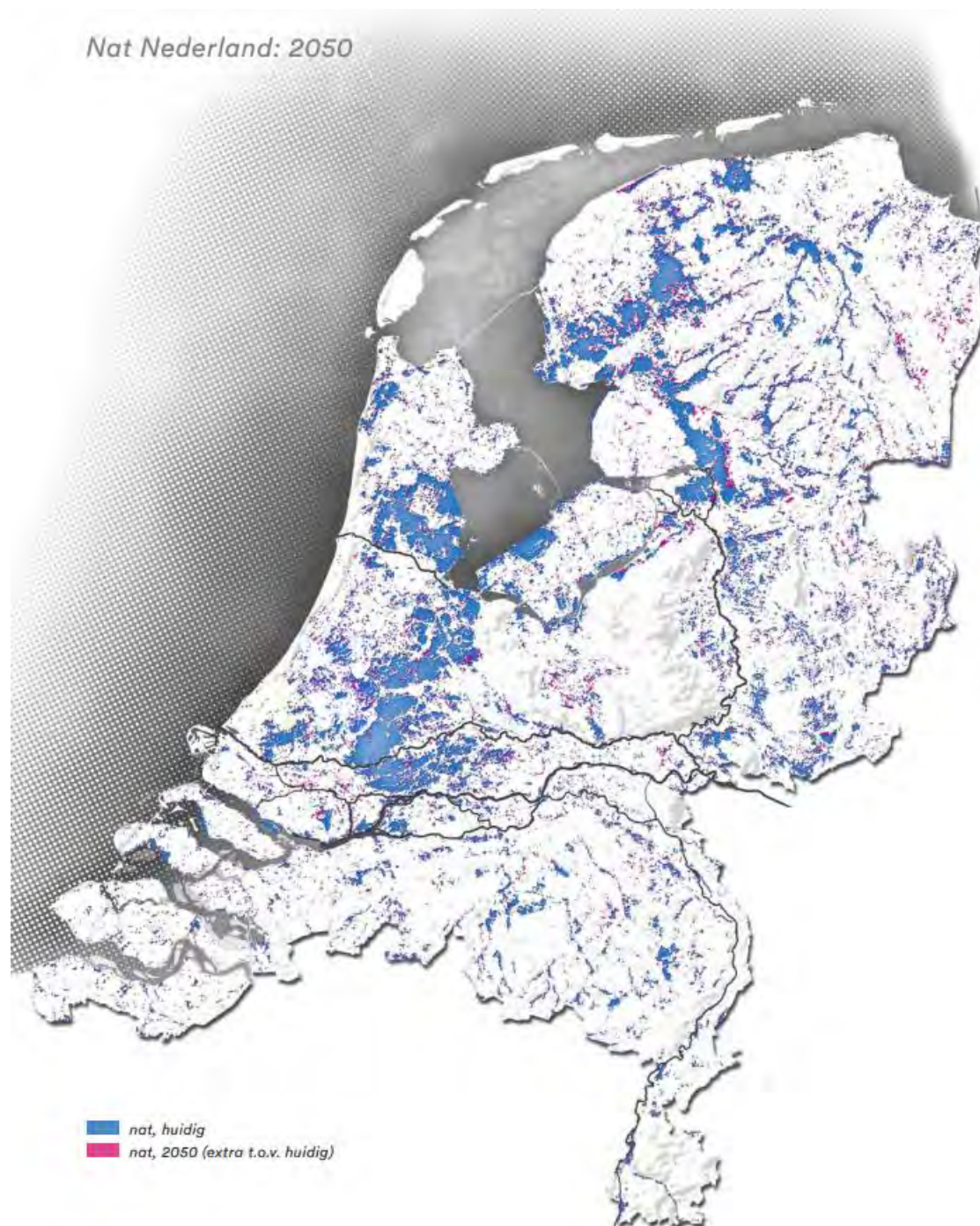
Figuur 4.15: Nat Nederland (Bron: Deltares, n.d.)
