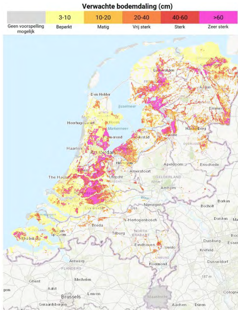
Figuur 4.10: Bodemdaling in 2100 in scenario 'hoog' (bron: Klimaateffectatlas)
