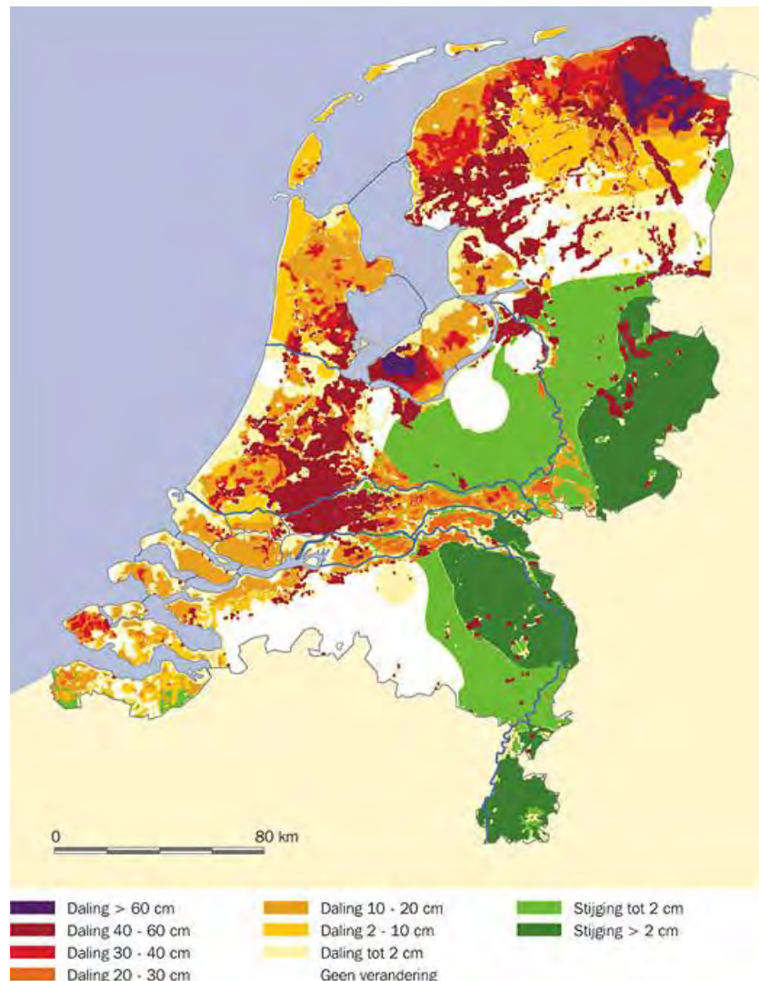
Figuur 4.9 Bodemdaling in 2050 (Bron: Bodemplus, n.d.)
