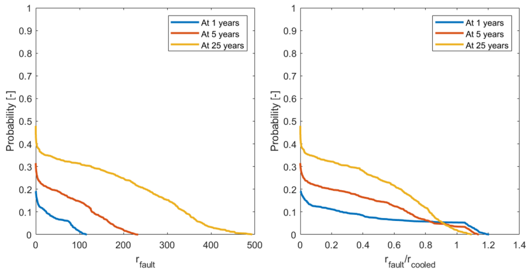
Figure 19 Probability of finding SCU > 1 at given distances to a fault (left) and at the relative distance (right). For distances larger than 1.2 times the cooled-zone radius, the stress is non-critical for all the cases.
