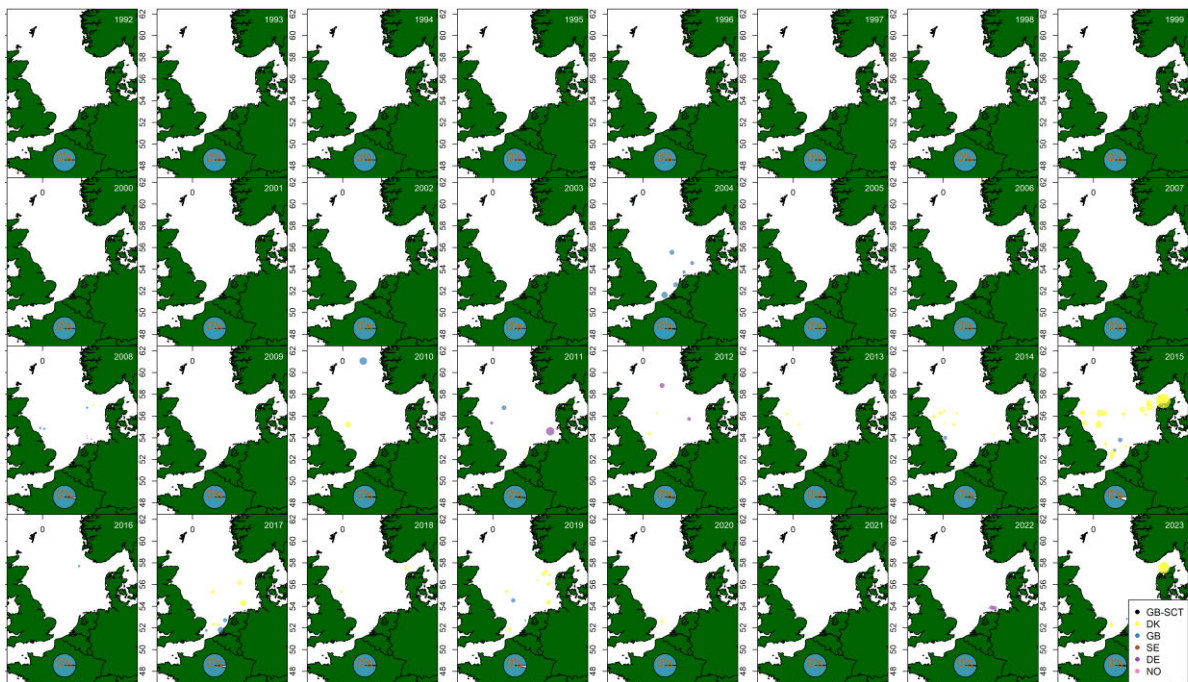
Figure A1-5: Distribution of catches of Loligo vulgaris in the NS-Q3.
